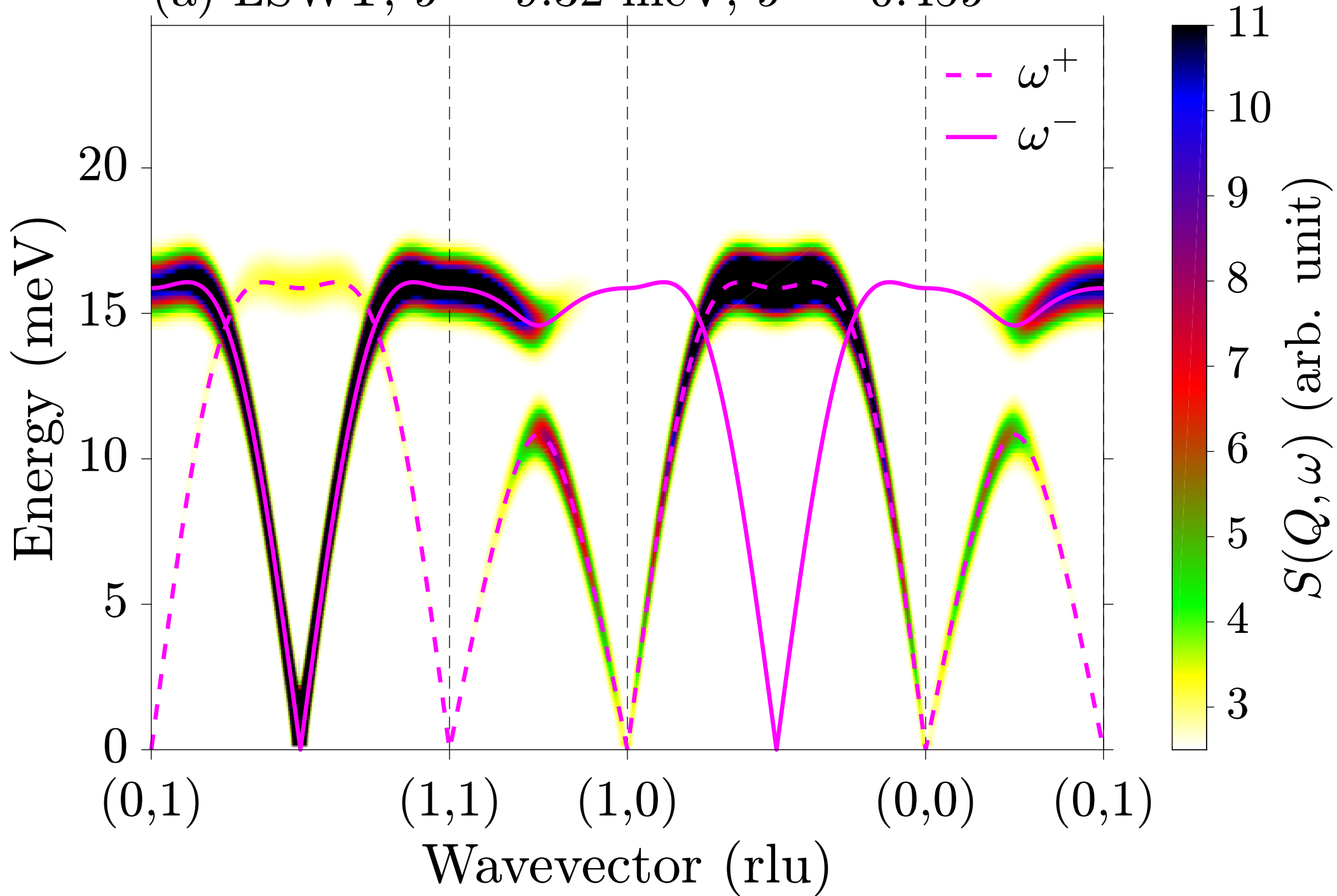
(a) LSWT, J = 9.32 meV, J' = 0.45J
